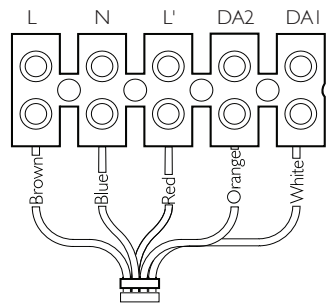
Figure 6: Wiring schematic
